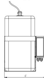
FRAME SIDE VIEW
